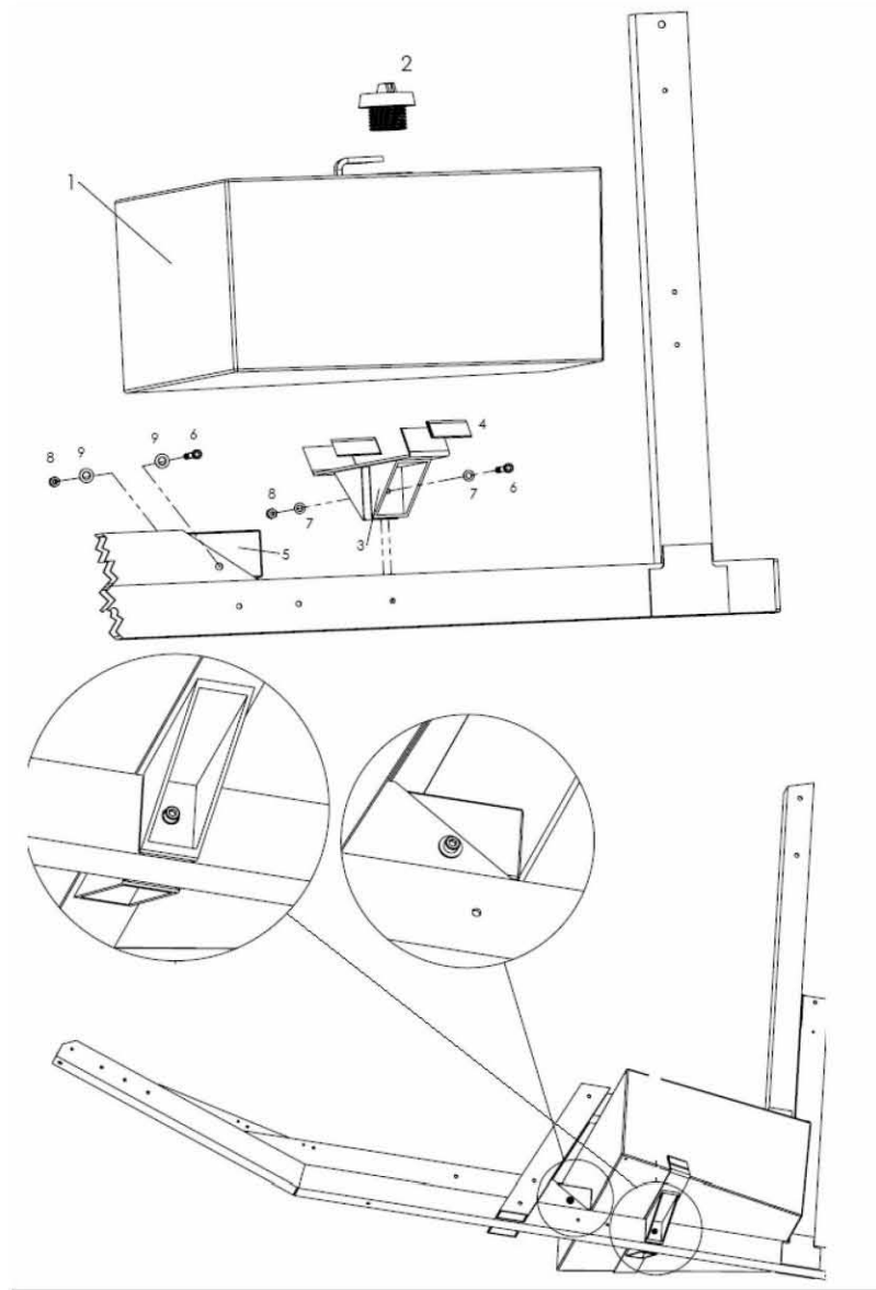
Fig-1 –Fuel tank
