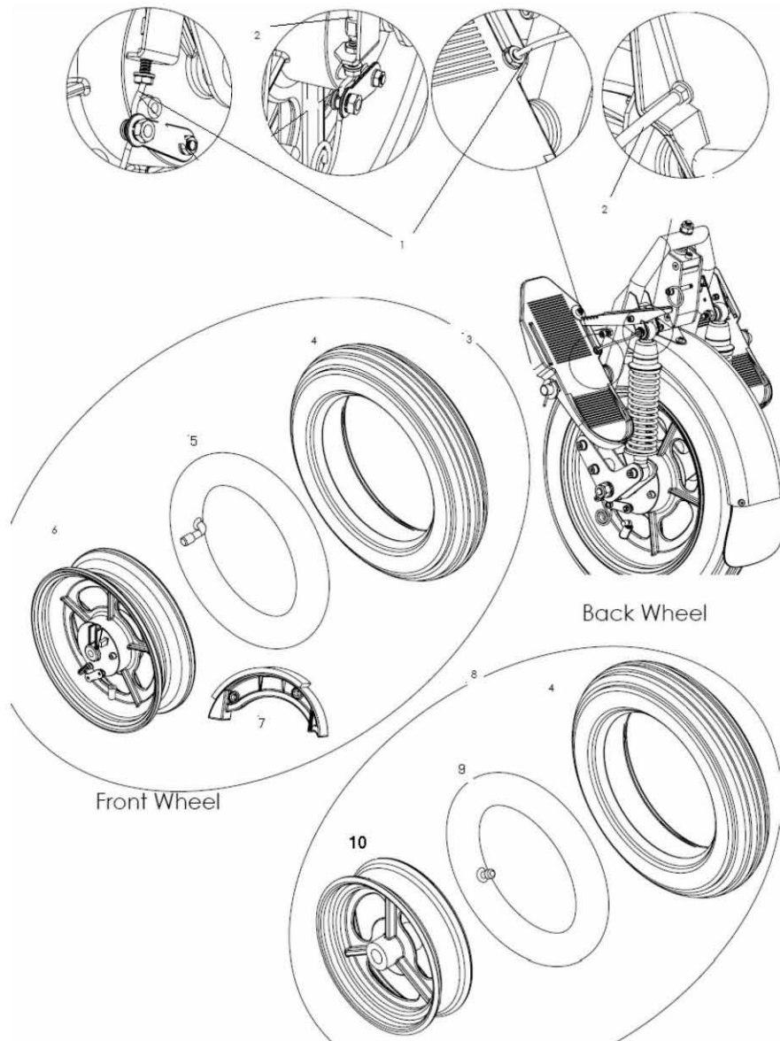
Fig-1 –Wheel and Brakes
