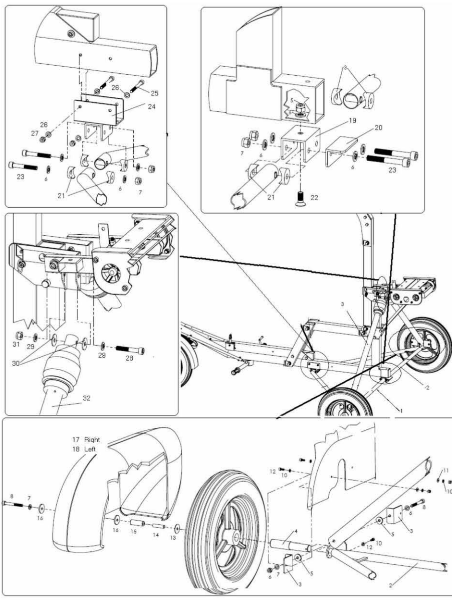
Fig-1 –Main Landing gear
