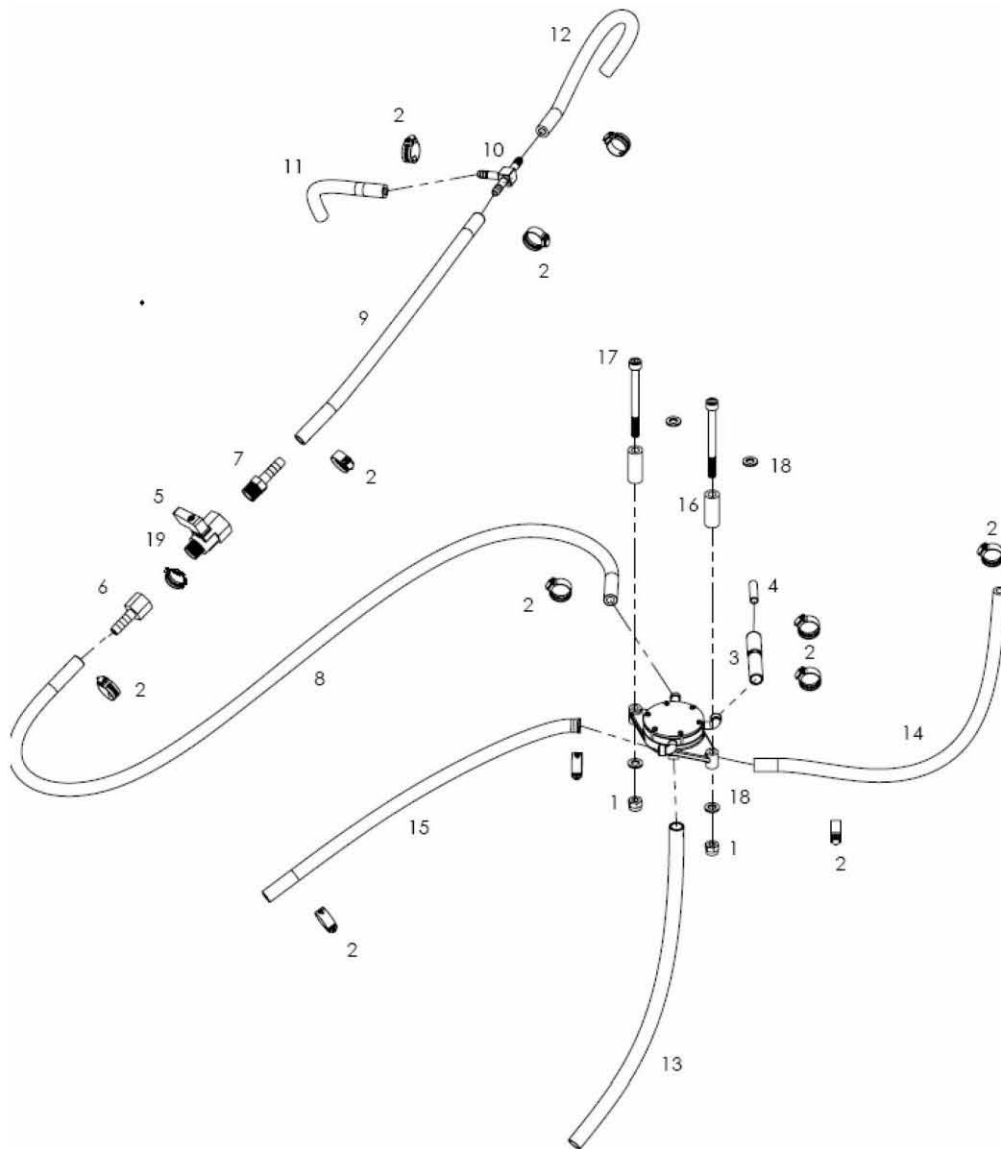
Fig-2 –Fuel Line
