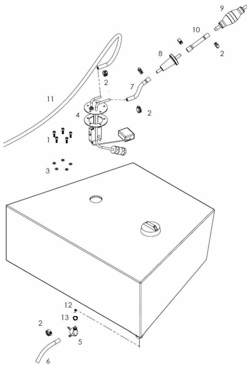
Fig-1 –Fuel Line
