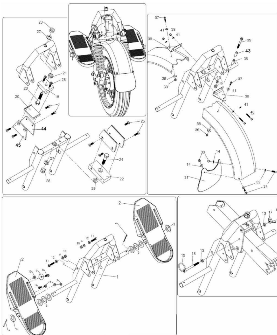
Fig-1 –Front Landing gear
