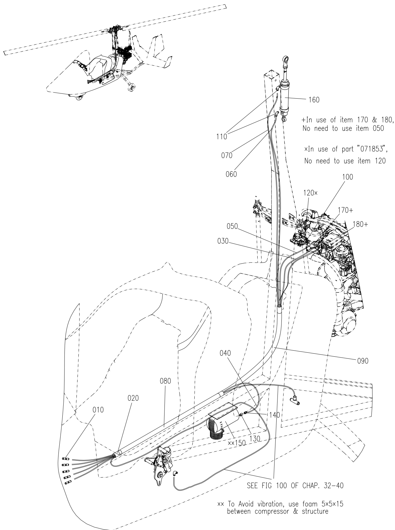
PNEUMATIC SYSTEM LINES ASSY.
