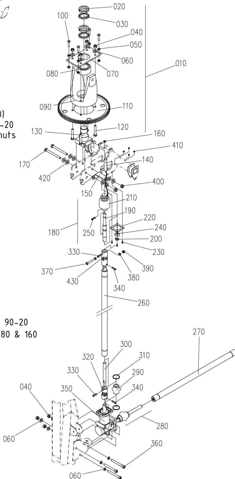
MAIN ROTOR GEAR BOX ASSY.
