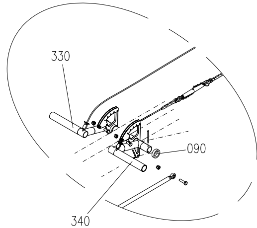
DETAIL E:
