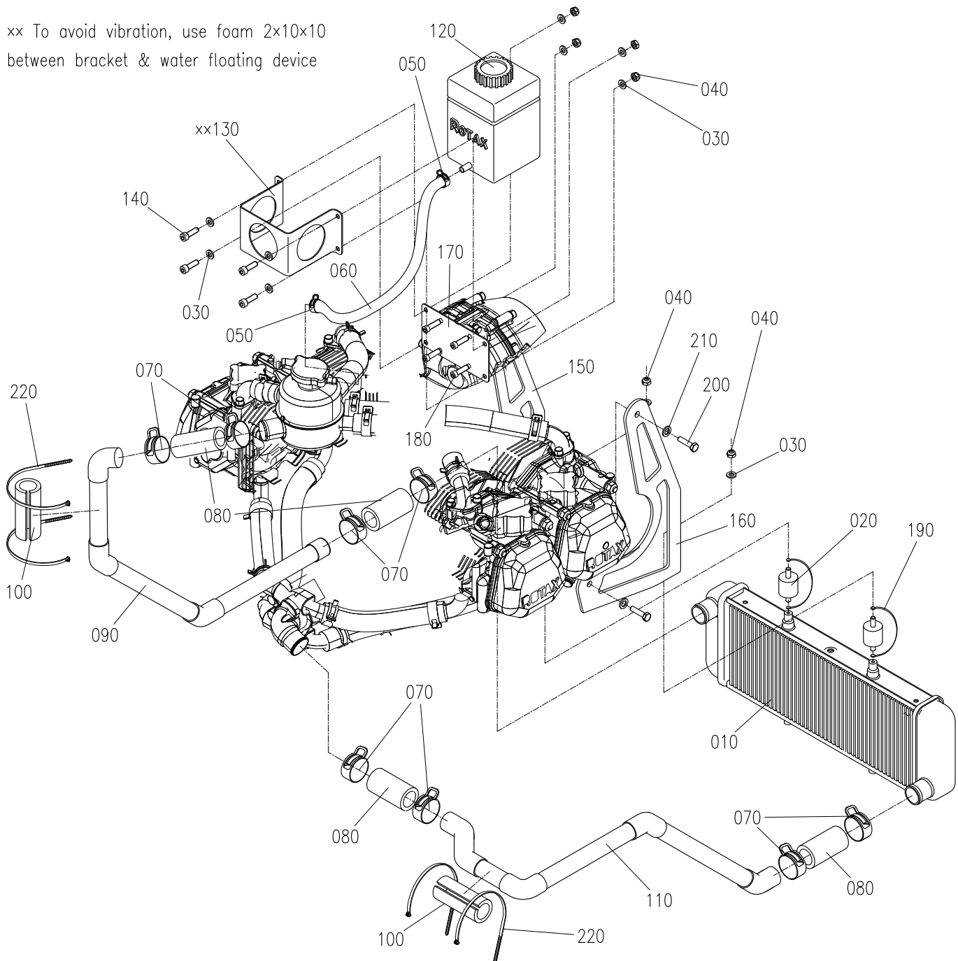
ENGINE COOLING SYSTEM ASSY.
