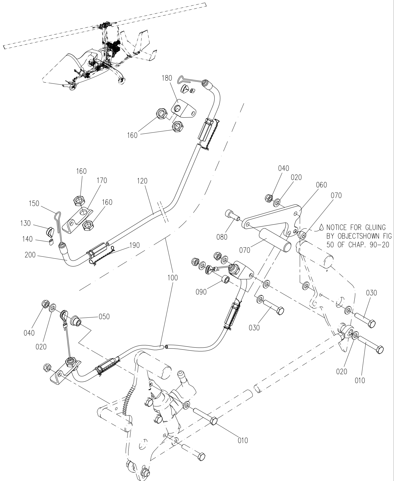
DUAL BRAKE SYSTEM ASSY – (OPTIONAL).
