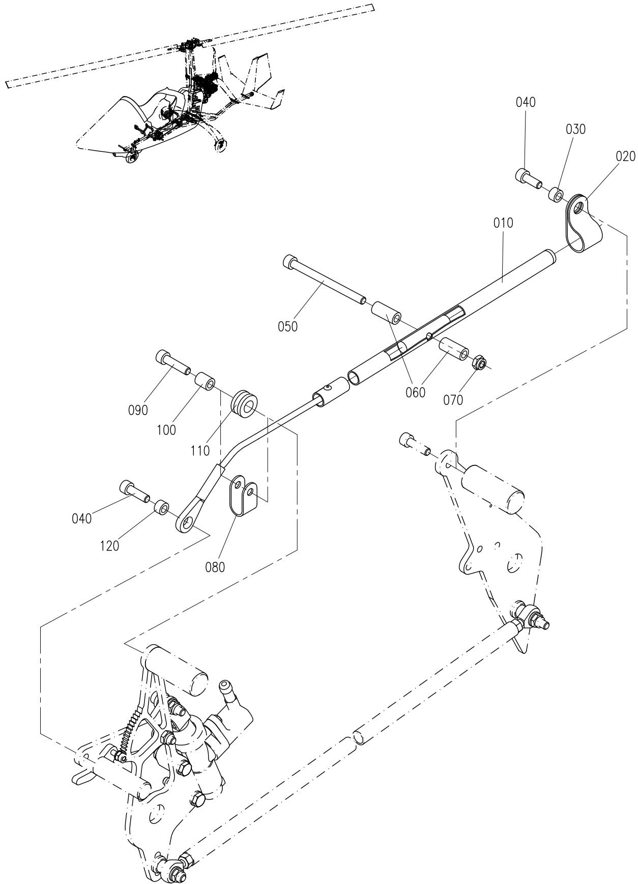
DUAL BRAKE SYSTEM ASSY – (OPTIONAL-2).
