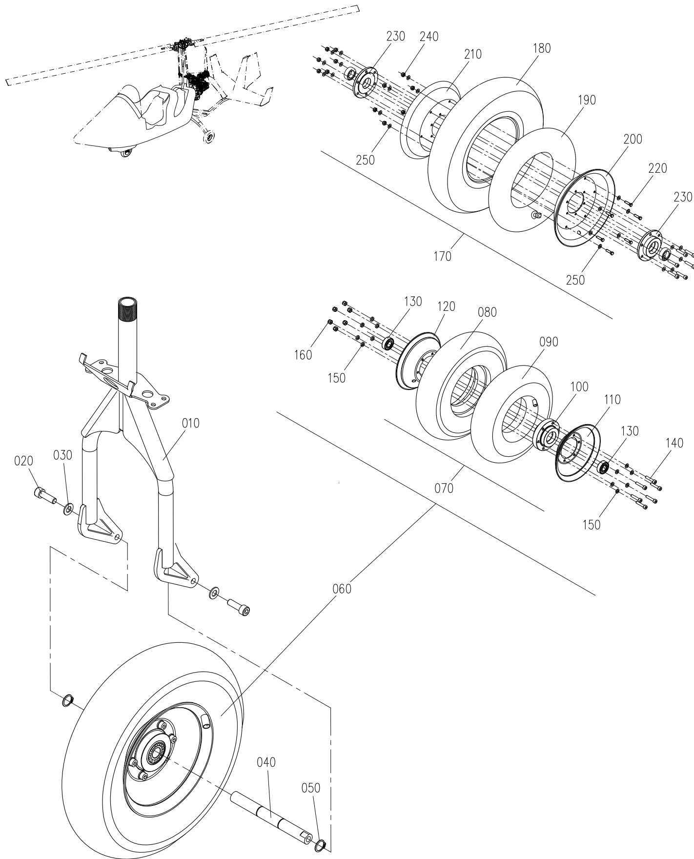
NOSE LANDING GEAR ASSY.
