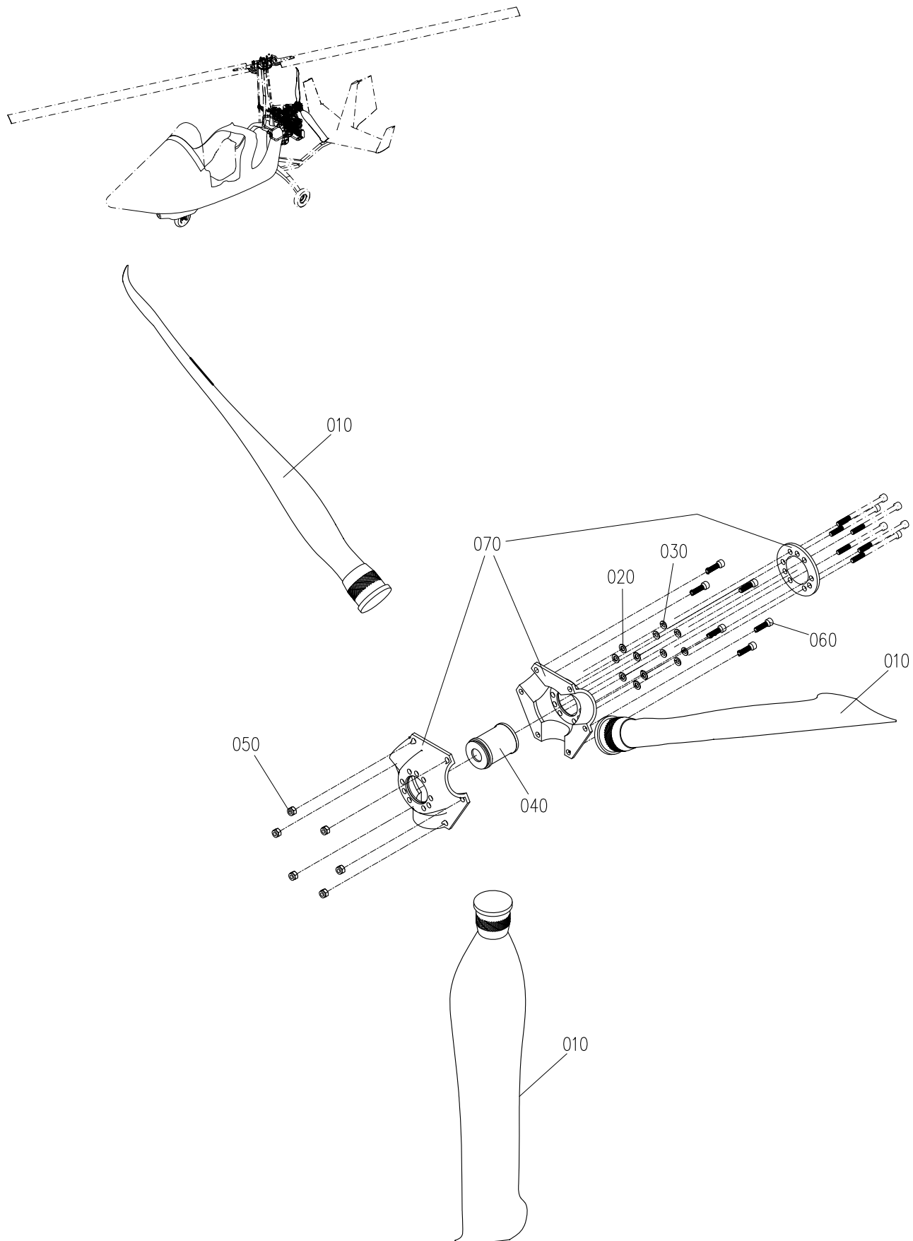
PROPELLER ASSY.
