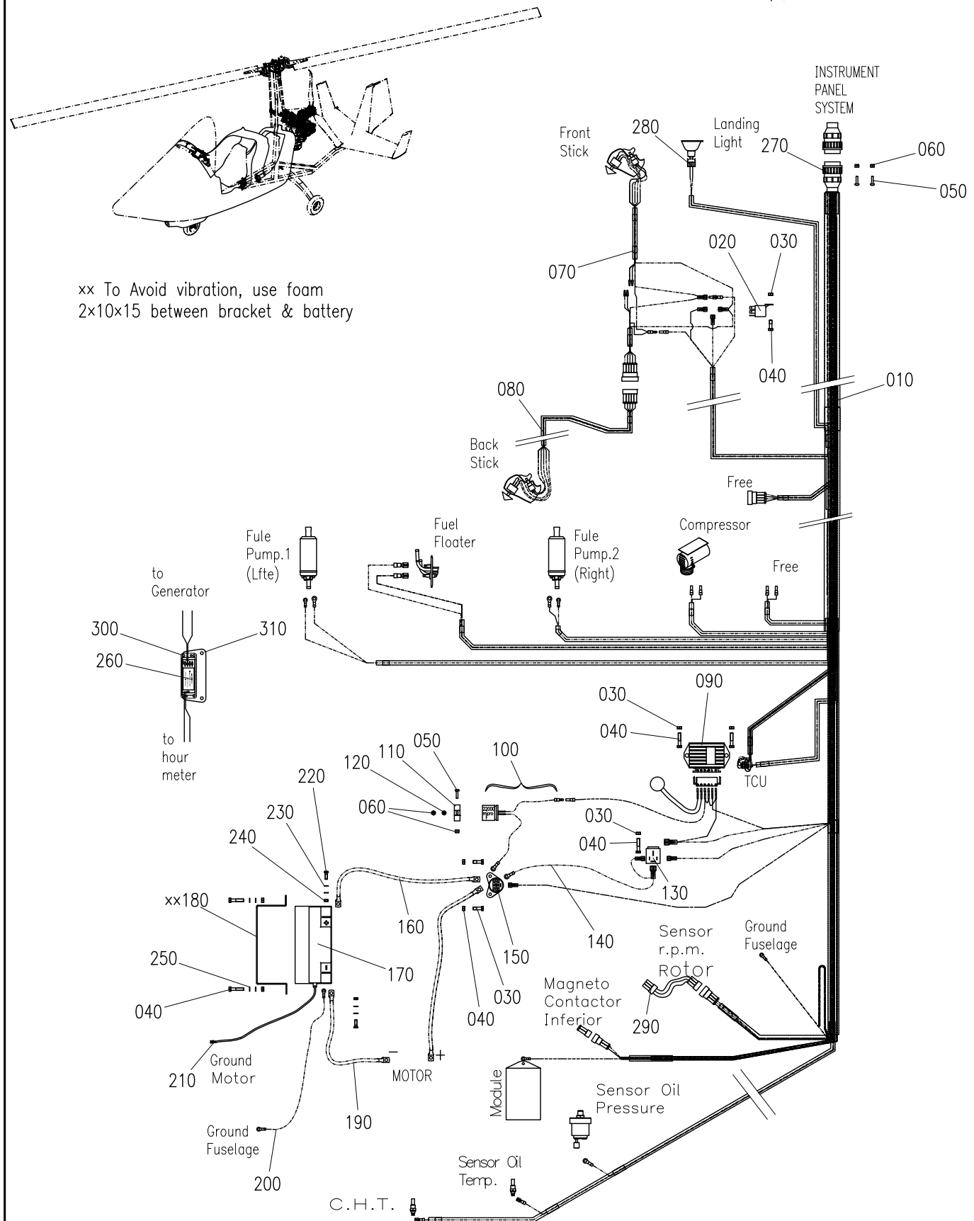
ELECTRIC SYSTEM WIRING ASSY.-FUSELAGE
