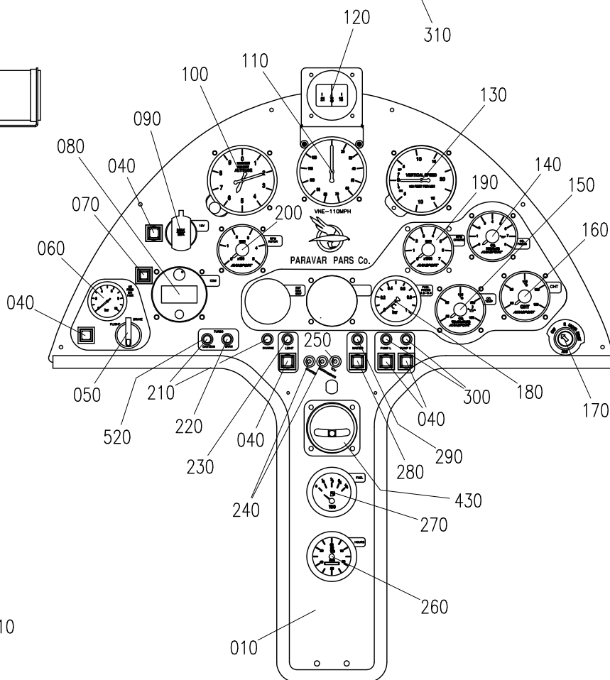
SYSTEM ELECTRICAL – PANEL ASSY.
