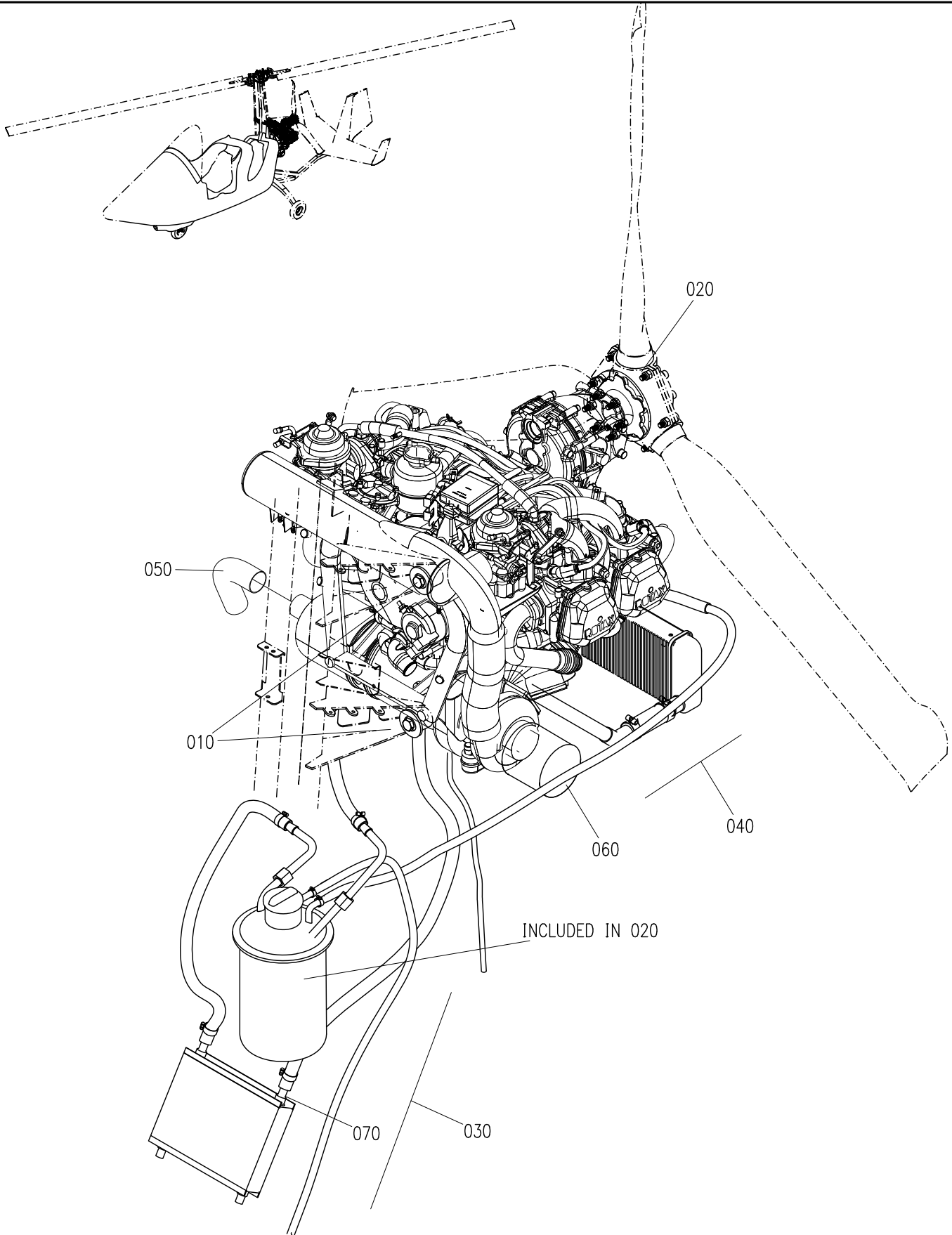
POWER PLANT INSTALLATION ASSY.
